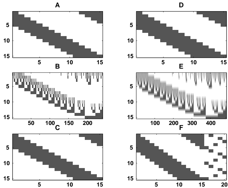
Figure 1: Permitted sets of the ring network. The ring network consists of 15 neurons with \alpha = 0.6 and \beta = 1 . In panels A and D, the 15 groups are represented by columns. Black refers to active neurons and white refers to inactive neurons. (A) 15 groups of width d = 5 . (B) All permitted sets corresponding to the groups in A. (C) The 15 permitted sets in B that have no permitted supersets. They are the same as the groups in A. (D) 15 groups with width d = 6 . (E) All permitted sets corresponding to groups in D. (F) There are 20 permitted sets in E that have no permitted supersets. Note that there are 5 spurious permitted sets.
